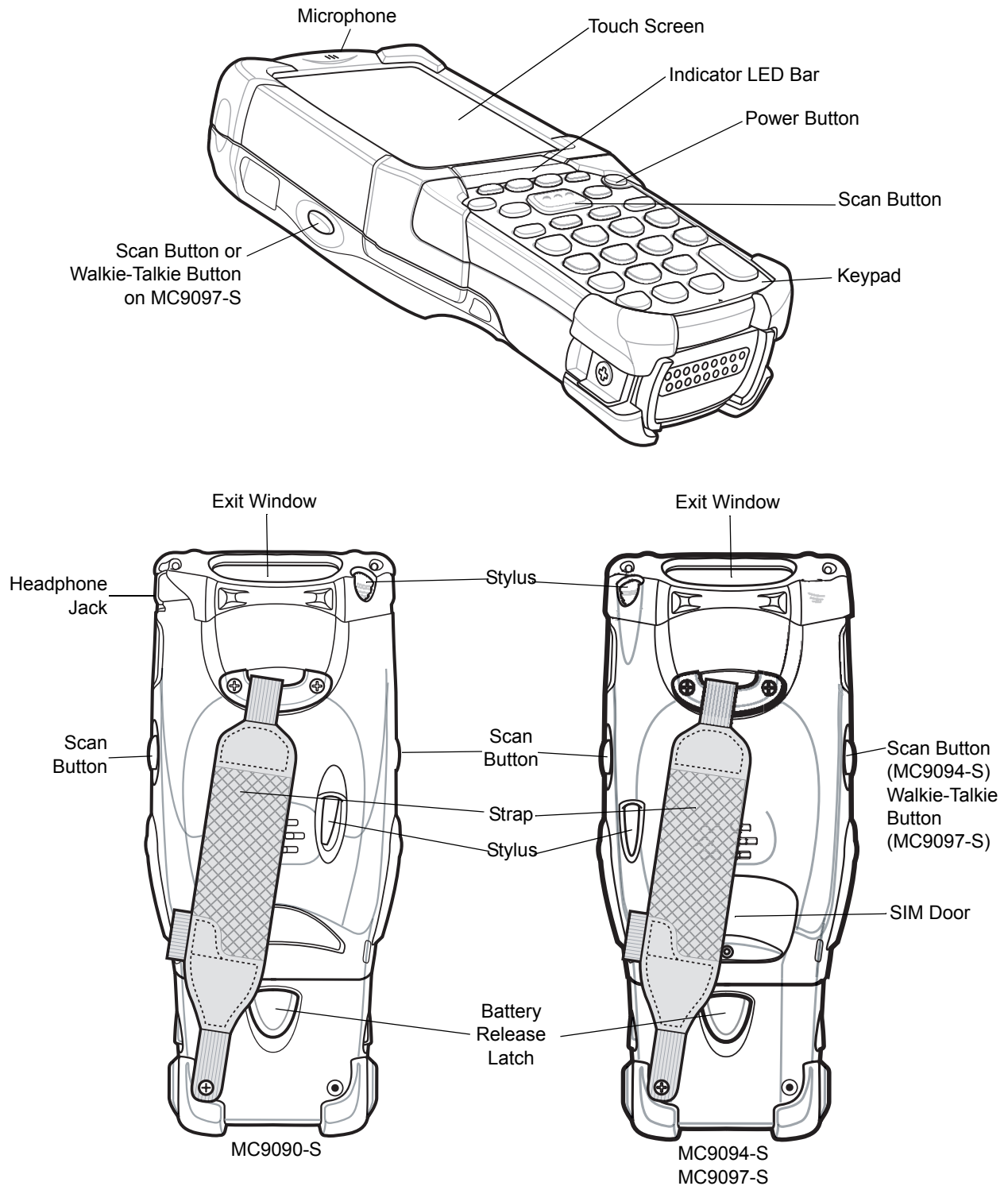
Figure 1-3 MC909X-S
